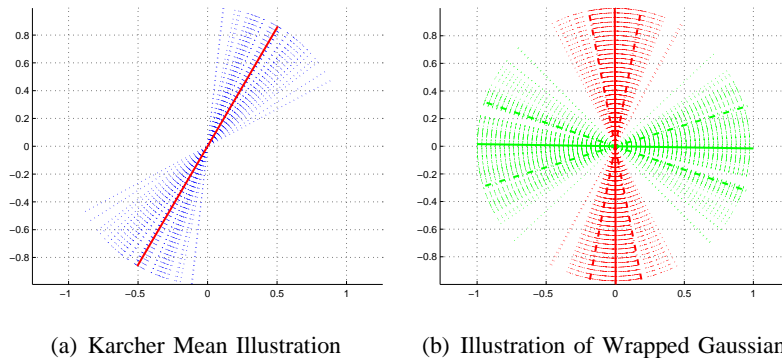
Fig. 3. In \mathbb{R}^2 the set of all axes (lines passing through the origin) is the Grassmann manifold with n = 2 and d = 1 .
